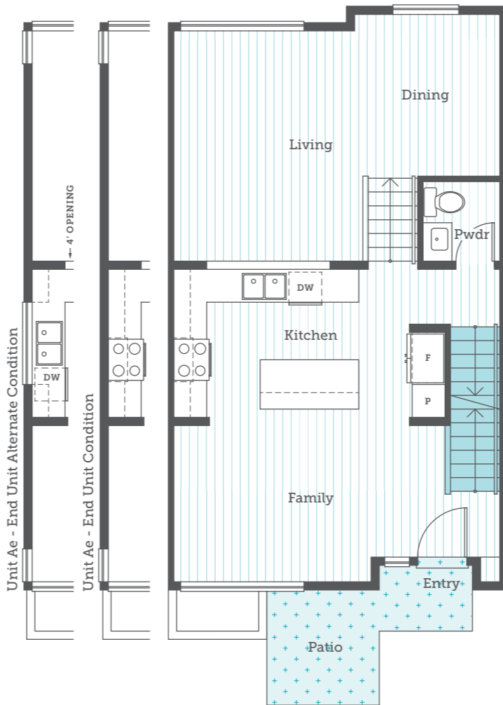
Main Floor 710 sqft
