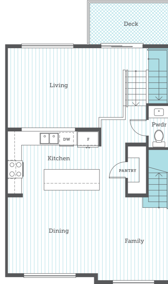
Main Floor 815 sqft
