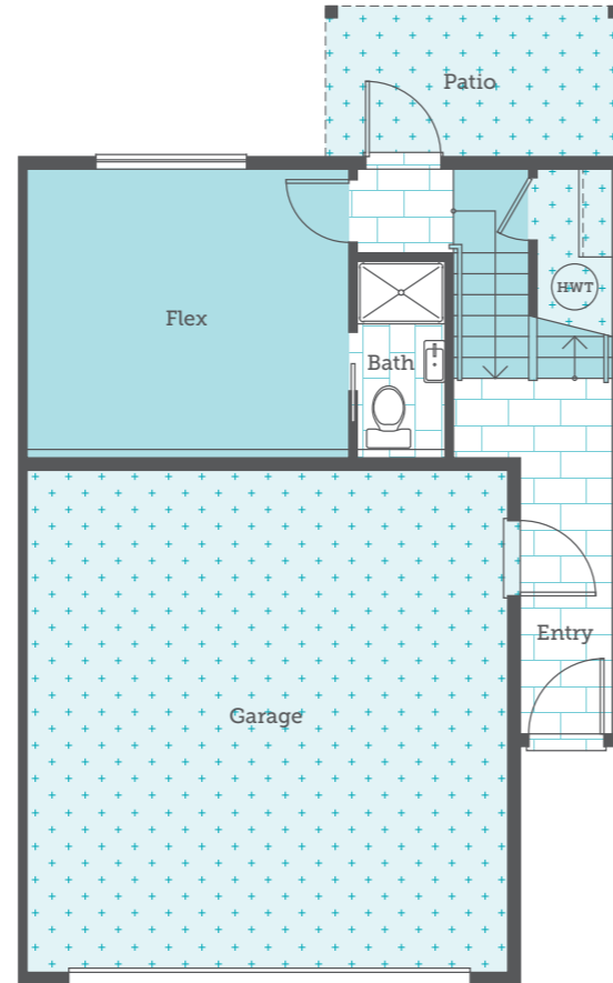
Ground Floor 344 sqft
