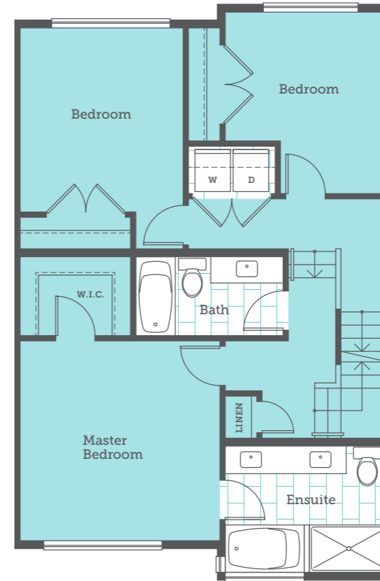
Upper Floor 887 sqft
